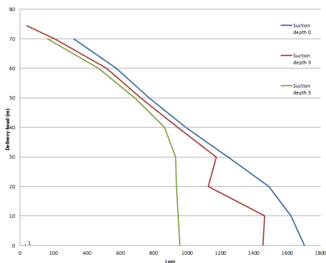
Delta Fire-fighting pump
